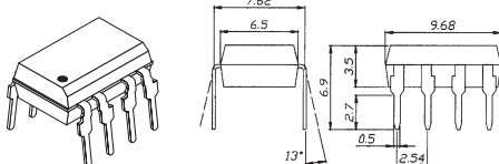
PDIP-8
